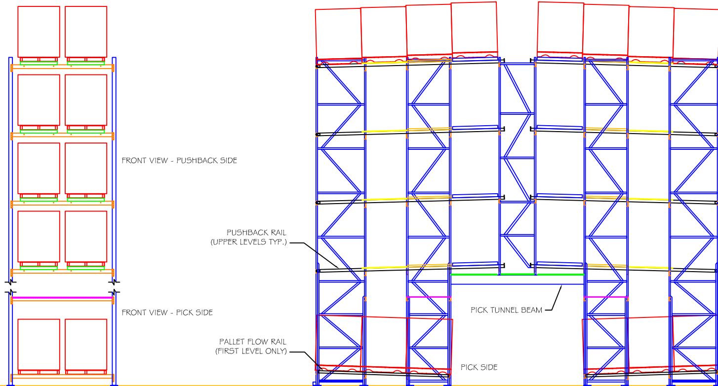
① 4 DEEP PUSHBACK W/ 3 DEEP PALLET FLOW - ENTRY/FRONT ELEVATION - 2 WIDE
